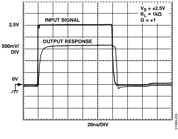
Figure 28. Input Overload Recovery, V_S = \pm 2.5 V
