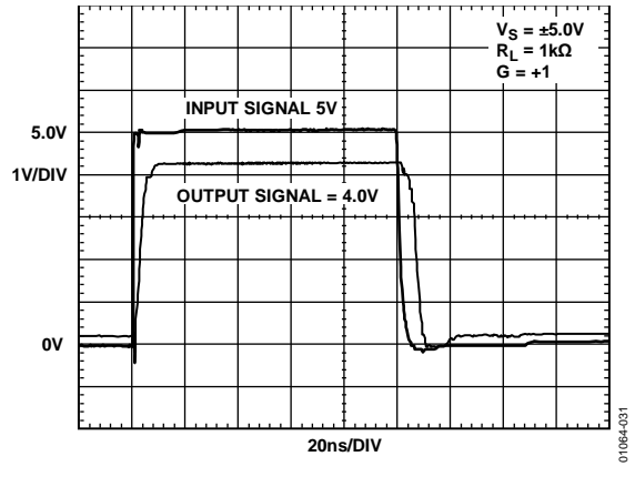
Figure 29. Output Overload Recovery, V_S = \pm 5.0 V
