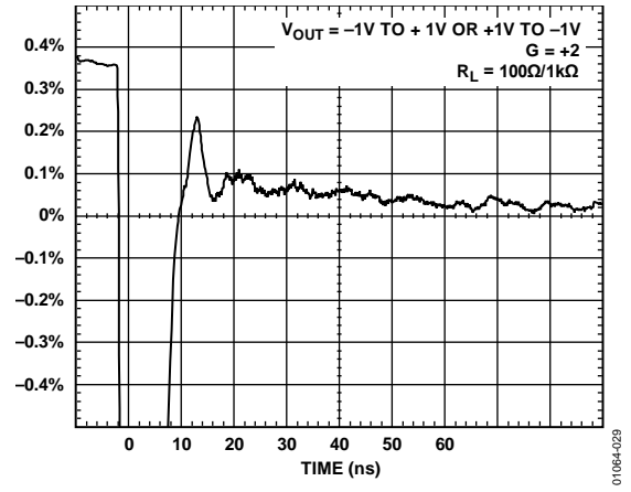
Figure 27. Settling Time
